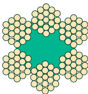
6X25 FILTER 1+6+6+12
